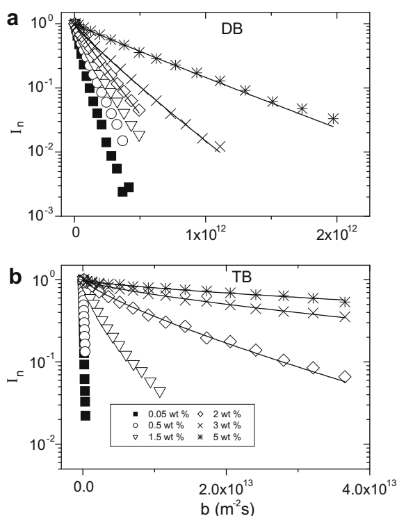
Fig. 7. Spin-echo attenuation in the systems and concentrations indicated. The curves are fits of Eq. (1) to the data. DB and TB denote diblock and triblock polymers, respectively. Redrawn from Ref. [10] with permission.
