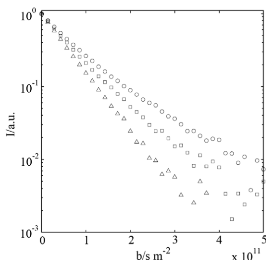
Fig. 2. A numeric solution to Eq. . The (normalized) echo intensities, I , are plotted vs. the field-gradient parameter b . Parameters used are: M_0 = 100 kDa, \alpha = 0.525 and K = 8.4 \times 10^{-9} \text{ m}^2 \text{ s}^{-1} . The polydispersity index is 1.1 ( \Delta ), 1.5 ( \square ) and 2 ( \circ ). A signal to noise ratio of 500:1 has been added to the data by generating normally distributed random numbers.
