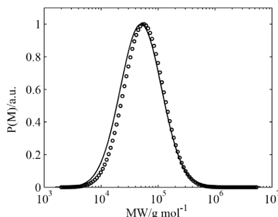
Fig. 4. The results of fitting Eq. to one of the echo-decays in . The solid line is the input distribution (with M_0 = 100 kDa and polydispersity index of 2) while ( \circ ) are the predictions of the fit. The parameters of the predicted distribution are: M_0 = 95.5 \pm 2.4 kDa and the value of the polydispersity index is 2.09 \pm 0.04 .
