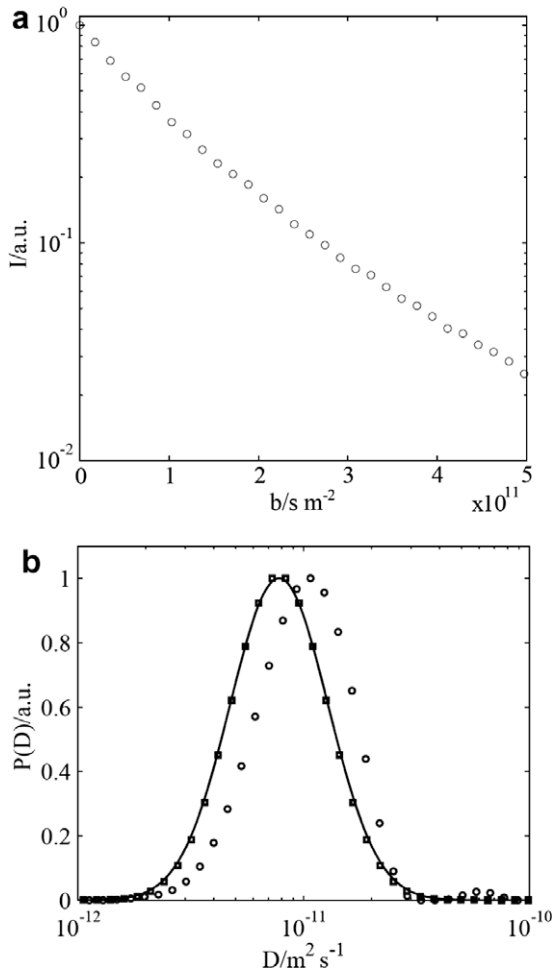
Fig. 5. (a) A calculated Stejskal–Tanner plot of echo intensity I versus the factor b in Eq. for a polymer described by a log-normal distribution in diffusion coefficients with D_0 = 1 \times 10^{-11} \text{ m}^2 \text{ s}^{-1} and \sigma = 0.5 , obtained from Eqs. (20a) and (20b). (b) The solid line is the input distribution of self-diffusion coefficients (DDC). Also shown are results of fitting the echo-decay in (a) to a log-normal form of DDC in Eq. (20a). The obtained parameters are: D_0 = 9.9 \times 10^{-12} \pm 0.07 \times 10^{-12} \text{ m}^2 \text{ s}^{-1} and \sigma = 0.49 \pm 0.013 . Also shown in (b) are the results of a Laplace inversion of the echo-decay ( \circ ).
